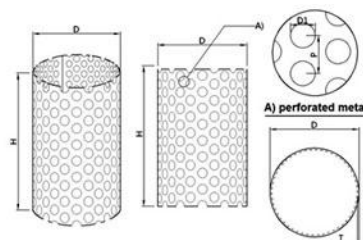
Perforated Metal Tube
