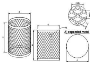
Expanded Metal Filter Tube
