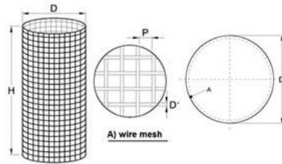
Woven Wire Mesh Cylindrical Filter
