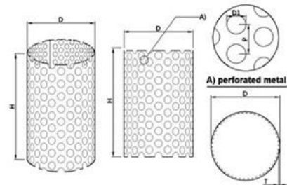
Perforated Metal Tube
