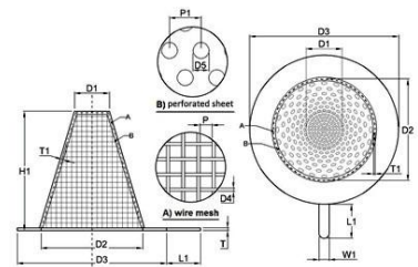
temporary basket strainer
