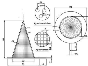
Conical Strainer
