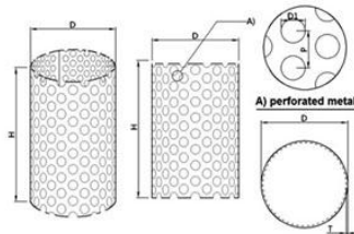
Cylindrical Screens
