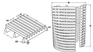
Filter baskets
